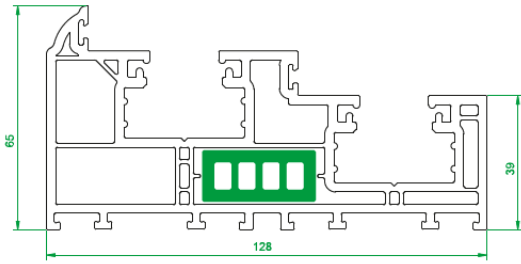
4001 Outer Frame
