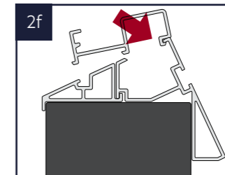
1. Fix the upper cladding back onto the ringbeam by clipping in the top edge under the lip.
