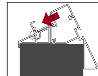
3. Finally, push the upper cladding towards the outside of the ringbeam so that the bottom clip engages.
