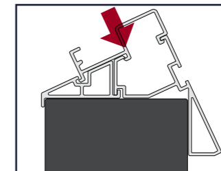
2. Tap the middle section of the upper cladding with a rubber mallet to ensure it clips into place.
