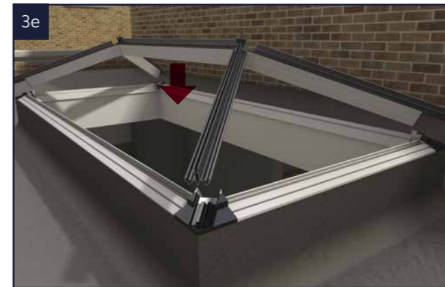
3e Lift the whole ridge assembly into place.
