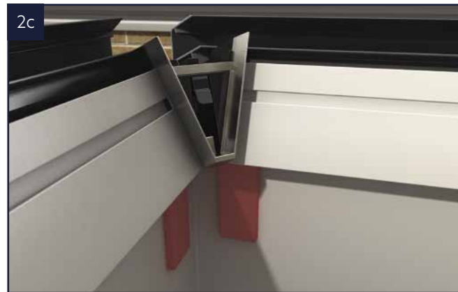
2c Ensure corners are tightly held against the aluminium. The corner connector assembly may need plastic packers behind if the upstand is not square or exact size.
